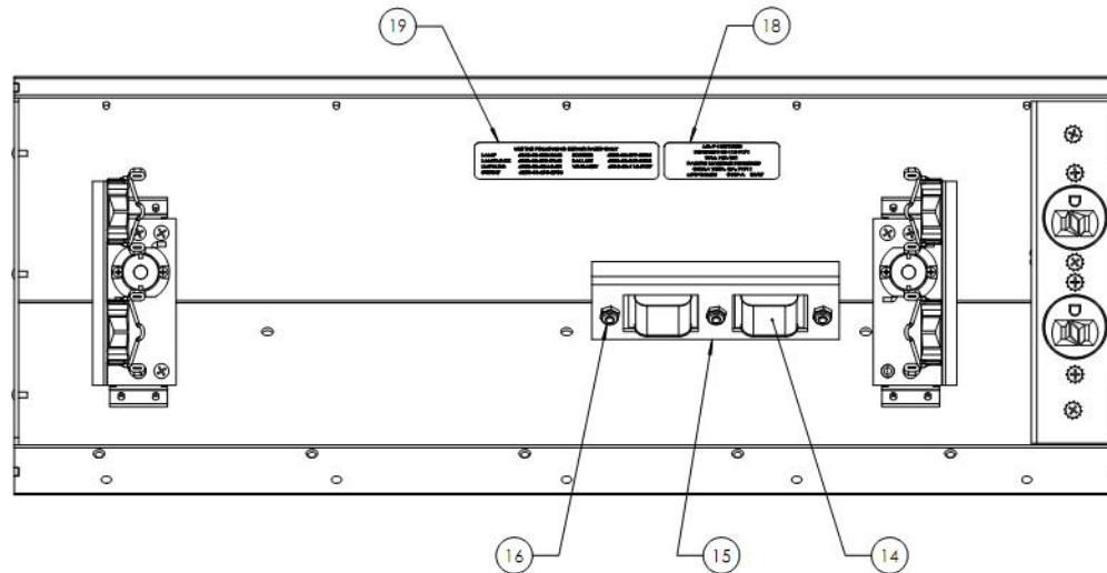
VIEW SHOWN WITH WINDOW FRAME, LAMPS AND REFLECTOR REMOVED FOR CLARITY
